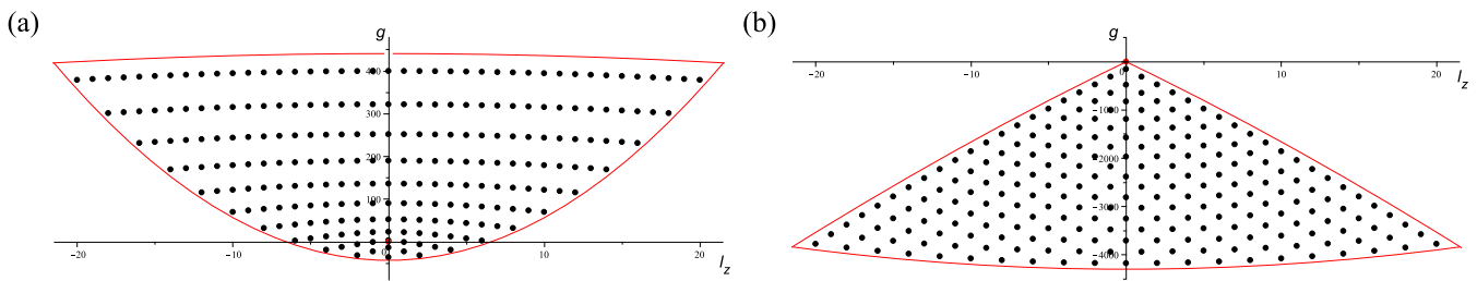
FIG. 8. Joint spectrum (l_z, g) of (\hat{L}_z, \hat{G}) (black dots) and classical critical values (red) for a = 1 (a) and a = 10 (b) and otherwise same parameters as in Fig. 7.
