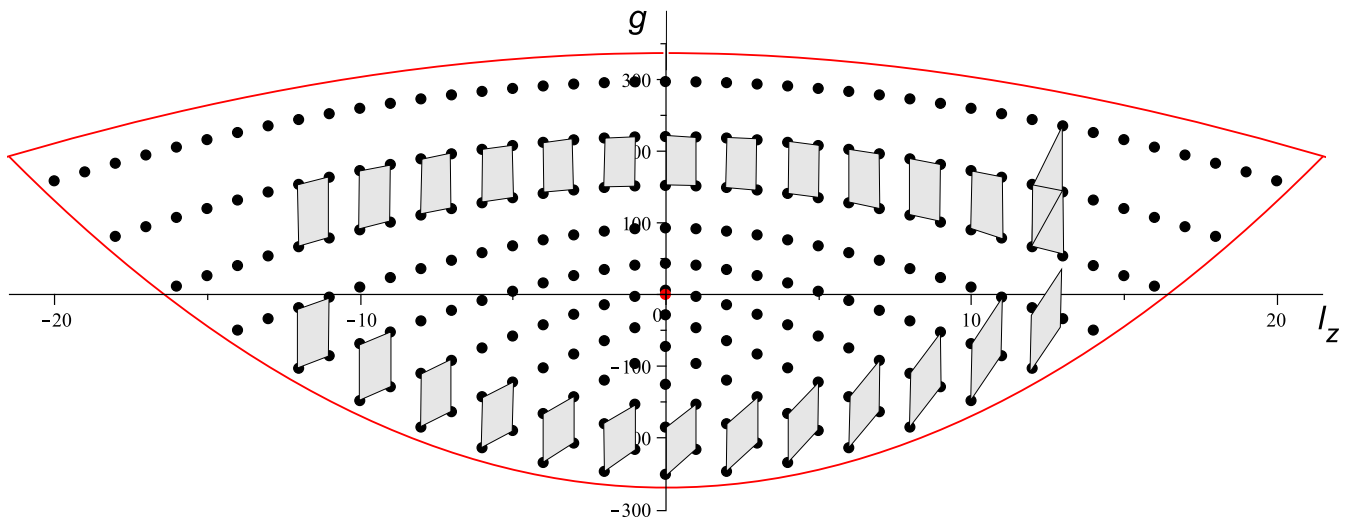
FIG. 7. Joint spectrum (I_z, g) of (\hat{L}_z, \hat{G}) (black dots) and classical critical values (red), for n = 20 , \omega = 1 , \hbar = 1 , and a = 3/2 . There are (n + 1)(n + 2)/2 joint states. The joint spectrum locally has a lattice structure which globally has a defect as can be seen from transporting a lattice cell around the isolated critical value at the origin.
